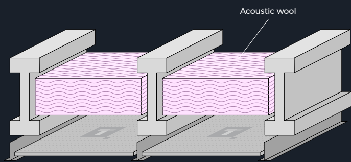
Scenario 1: Installation of T|Karra tiles with a minimum spacing of 6” between the joists and suspended ceiling.
